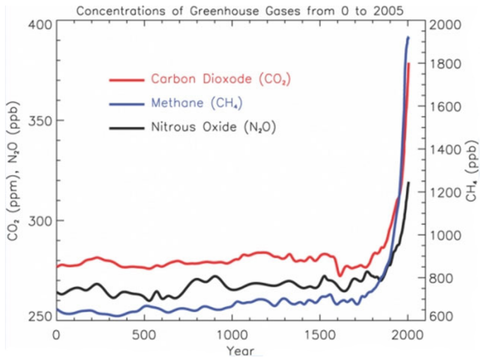
Graph #2: Greenhouse Gas Levels within the Last 2,000 Years
