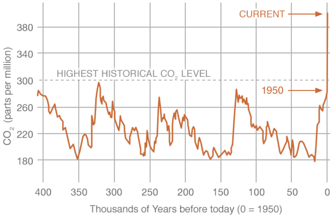
Graph #1: CO 2 Levels within the Last 400,000 years
